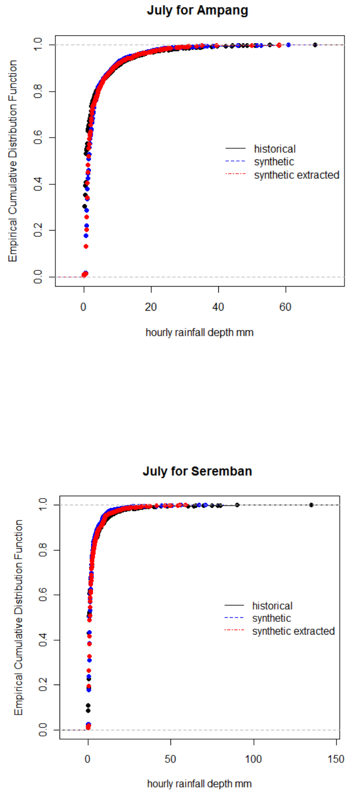
Figure 3. Comparison of the distribution function for historical, synthetic and synthetic extracted hourly rainfall for July for Ampang and Seremban stations
