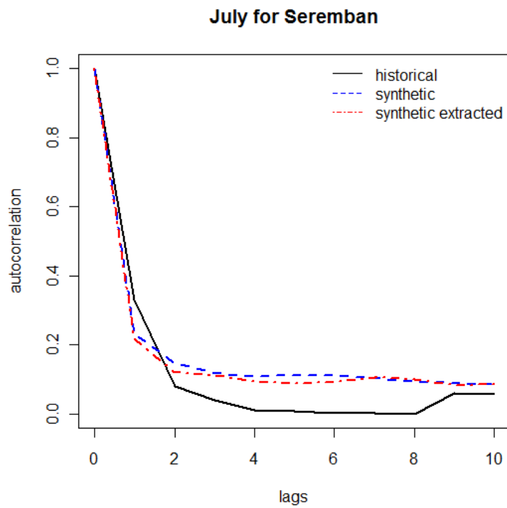
Figure 5. Comparison of autocorrelation function for historical, synthetic and synthetic extracted hourly rainfall for July for Ampang and Seremban stations
