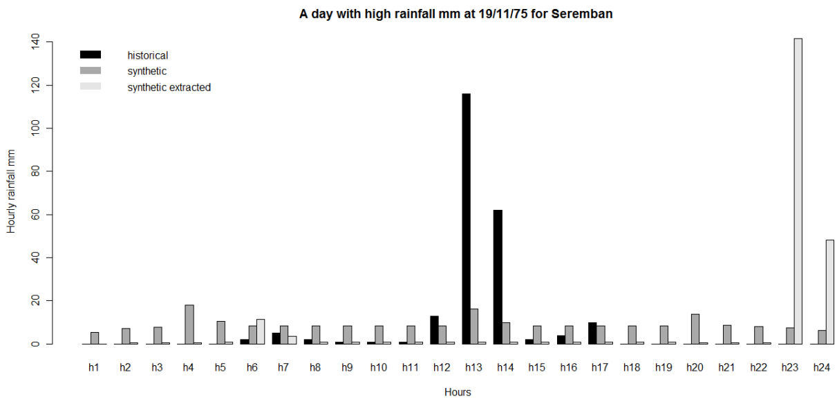
Figure 8. Comparison of hyetographs for historical, synthetic and synthetic extracted hourly rainfall for July and November for Seremban station
