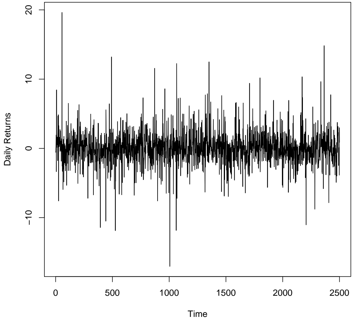
Figure 1: Plot of the simulated returns showing its evolution.
