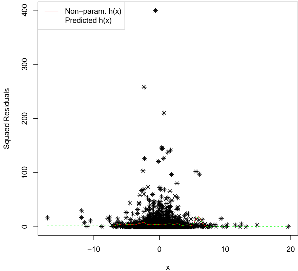
Figure 3: Graph of the variance h(\cdot) function and the predicted mean function of the simulated returns.
