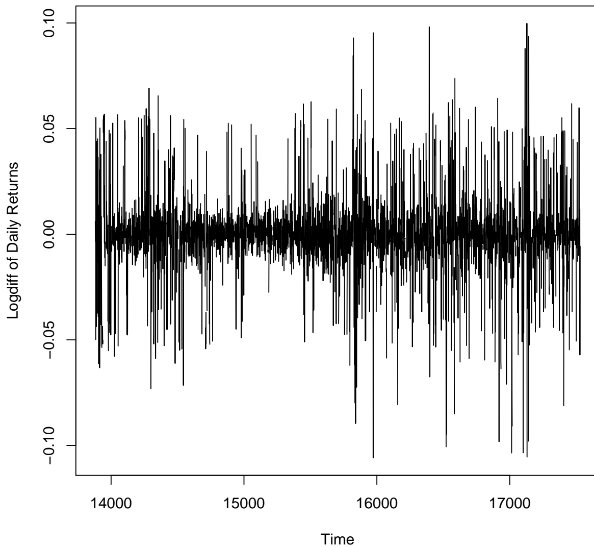
Figure 5: Graph showing the evolution of TOTAL's daily log difference of returns.
