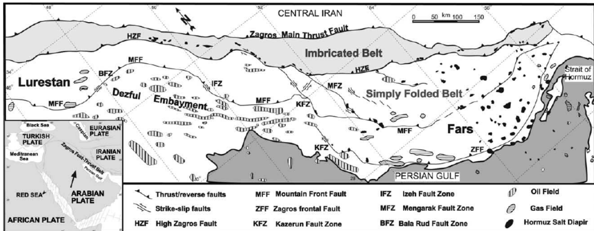
Figure 7: Structural setting of the Zagros fold-thrust belt showing the major fault zone [from 20]
