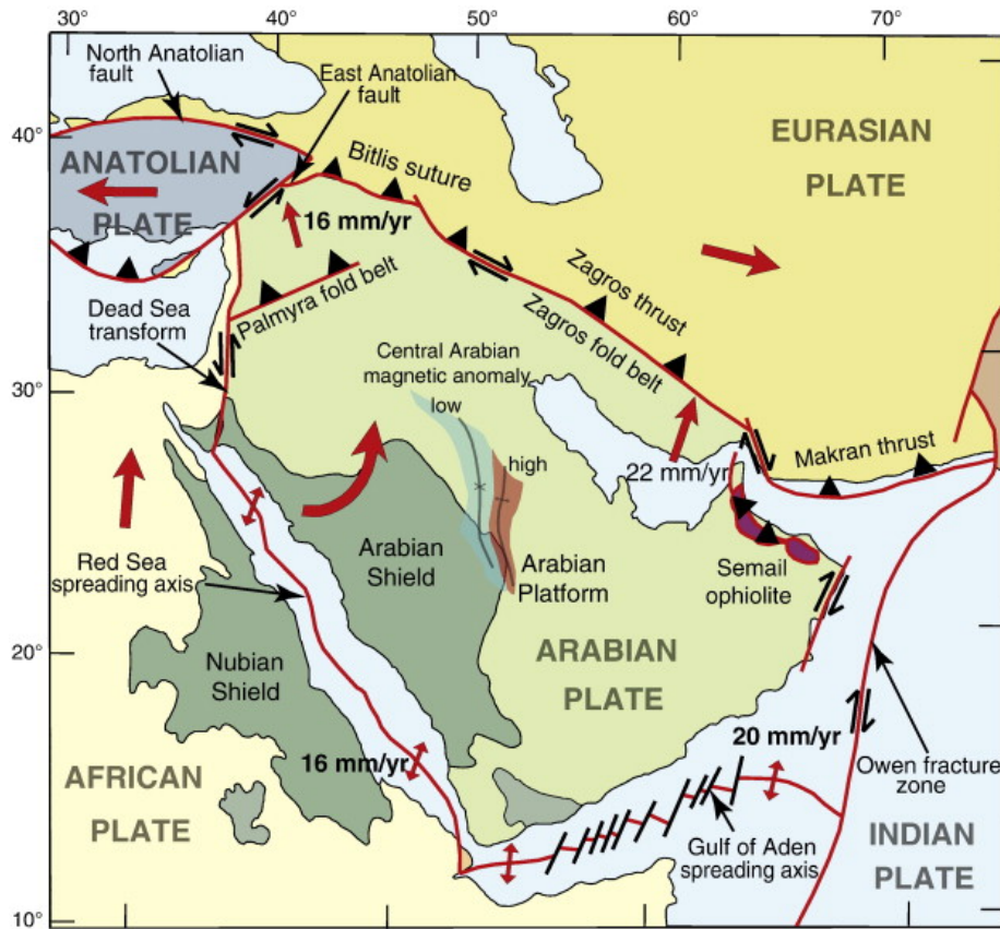
Figure 2: Main Tectonic sub-division of the Arabian plate and Location of Iraq ( http://africa-arabia-plate.weebly.com/arabian-plate.html ).
