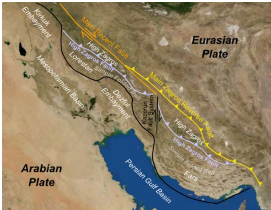
Figure 6: Tectonic Map of Zagros belt, shows the lateral divided laterally zones into four longitudinal segments ( https://en.wikipedia.org/wiki/Zagros_fold_and_thrust_belt )
