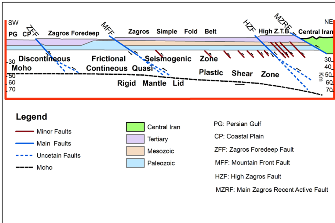
Figure 5: Simplified transverse cross section of the Zagros active fold-thrust mountain belt [modified after 3]
