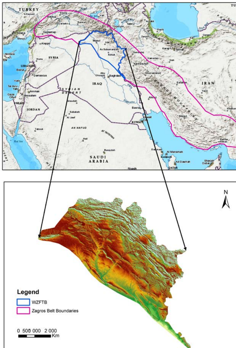
Figure 3: Location of the study area in Iraq.
