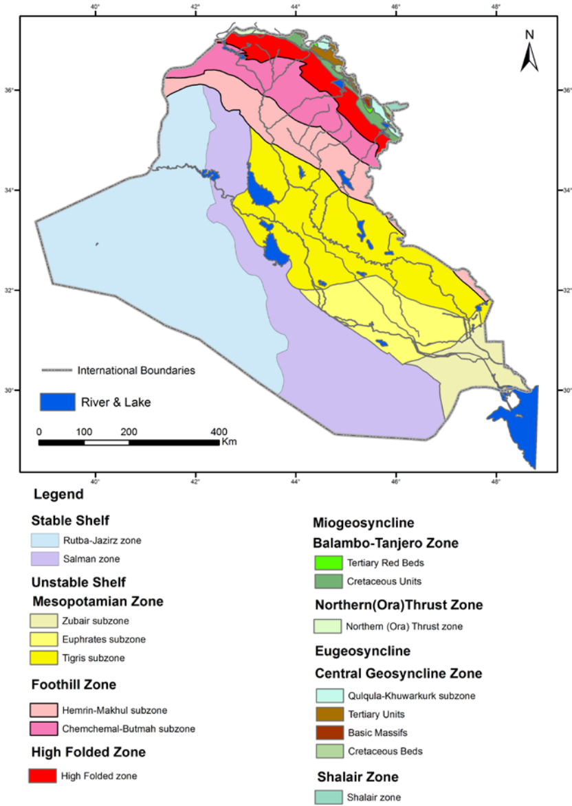
Figure 8: Tectonic Map of Iraq [modified after 26]
