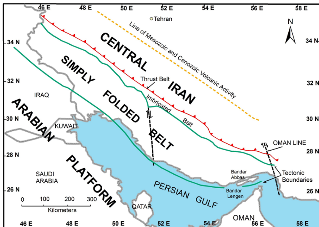
Figure 4: Tectonic settings of the Zagros fold and thrust belt showing the major tectonic belts [modified after 17]
