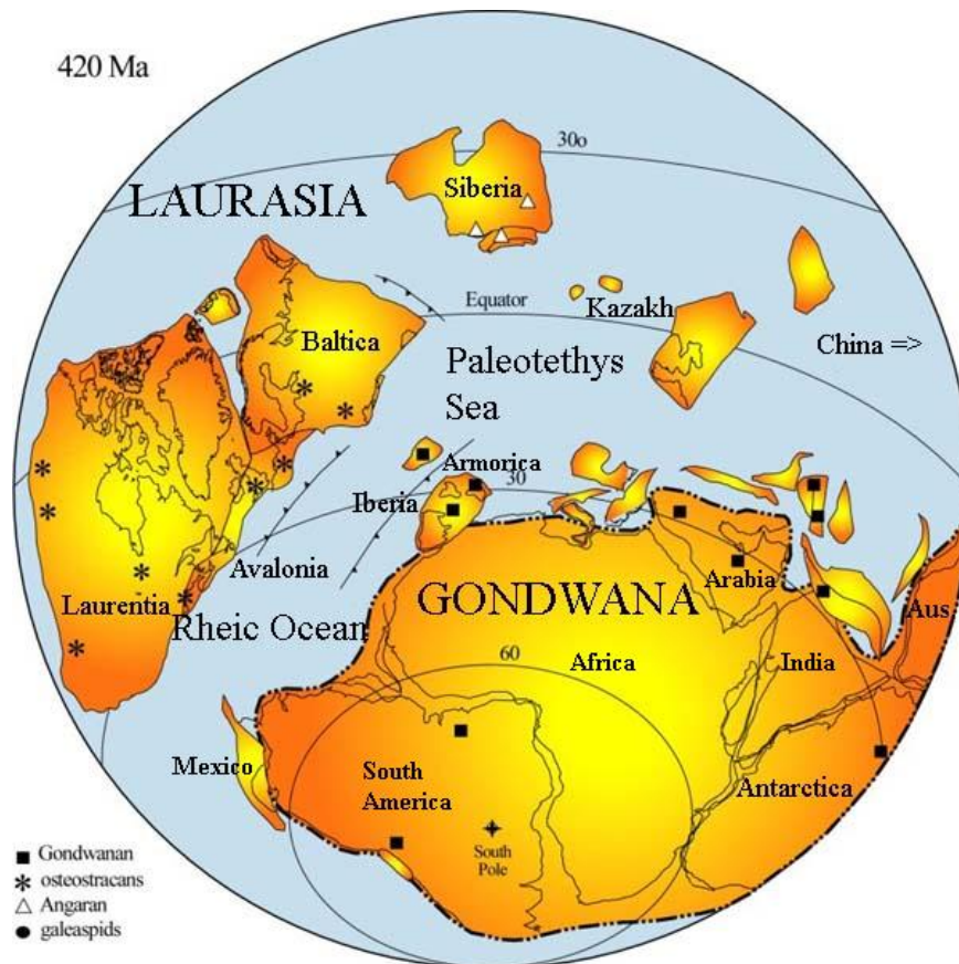
Figure 1: Supercontinent GONDWANA, early Paleozoic ( http://kingofwallpapers.com/gondwana.html ).
