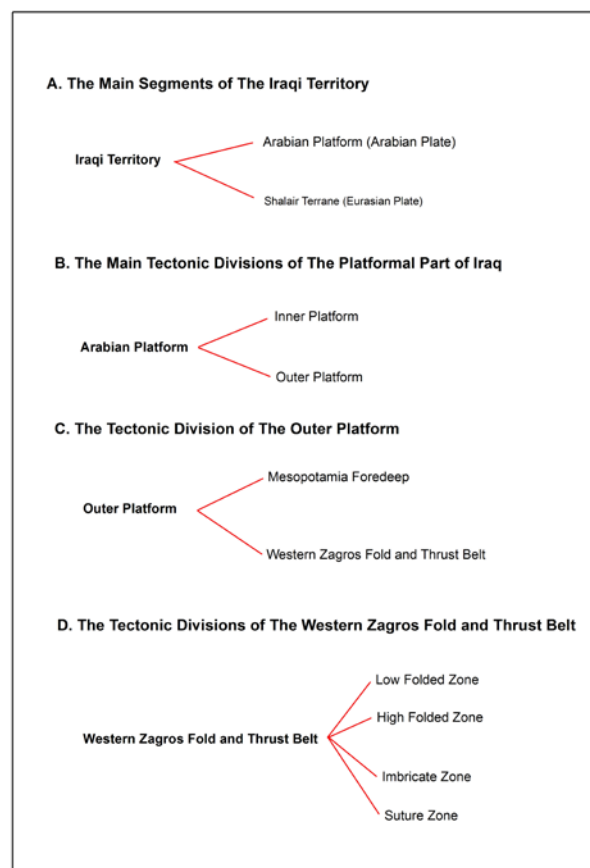
Figure 12: The Tectonic Divisions of Iraq [from 28]
