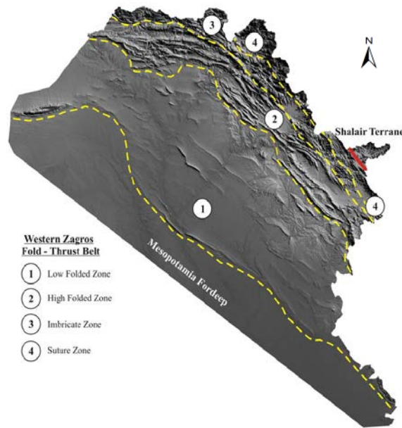
Figure 14: The tectonic subdivisions of the western Zagros fold and thrust belt [from 4]
