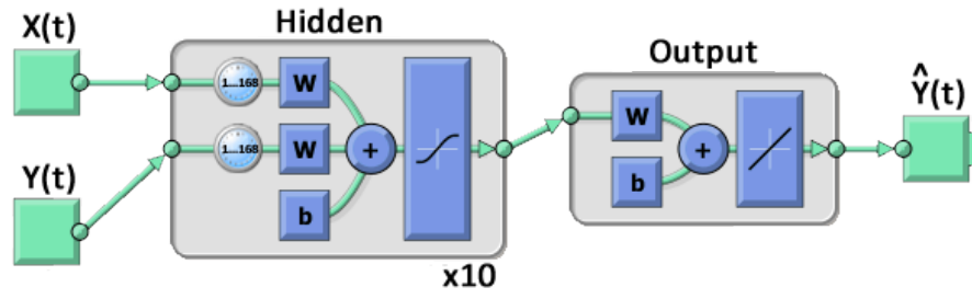
Figure 3- Artificial Neural Network architecture
