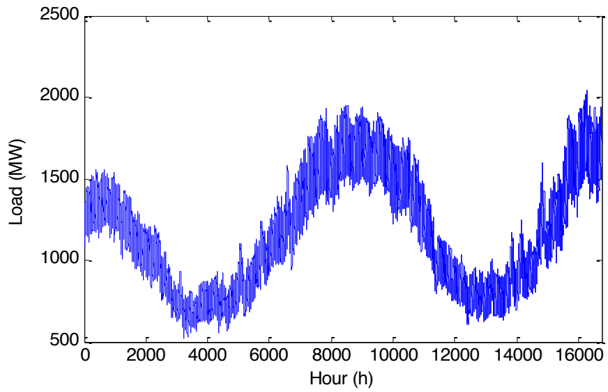
Figure 1- Electricity demand
