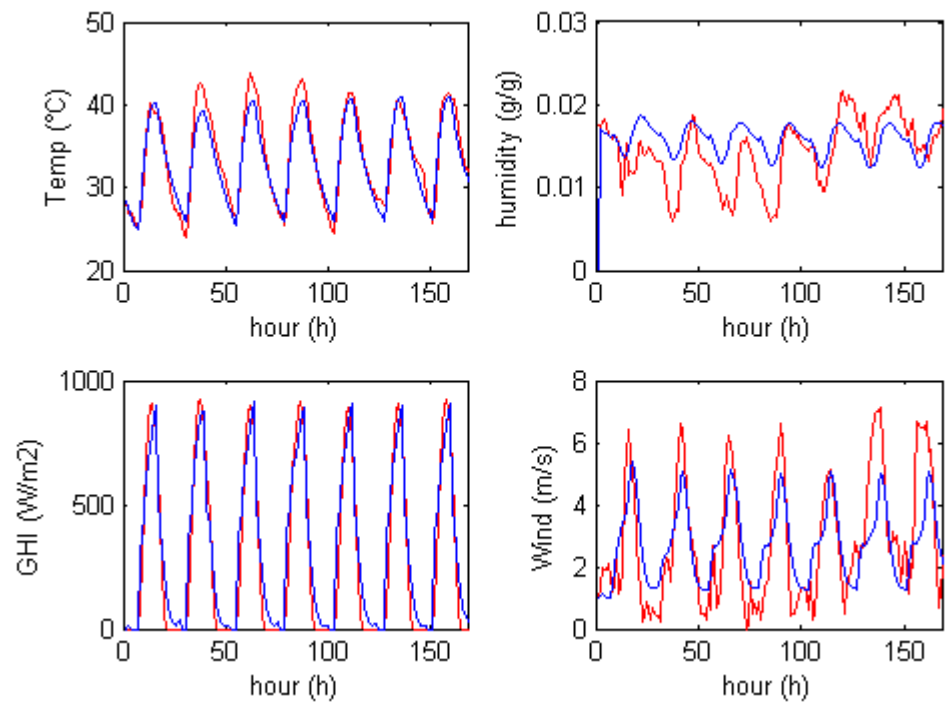
Figure 10- Predicted weather variables (blue) against measured (red)
