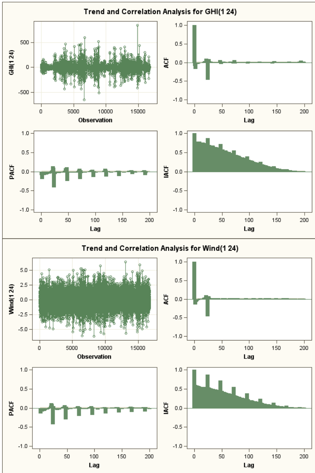
Figure 4- Trend and correlation analysis for 1-lag/24-lag differenced temperature (a), specific humidity (b), GHI (c) and wind speed (d)
