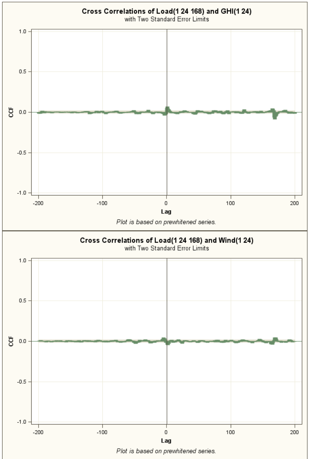
Figure 5 – Cross-correlation between 1-lag/24-lag/168-lag differenced load and 1-lag/24-lag differenced temperature (a), specific humidity (b), GHI (c) and wind speed (d)
