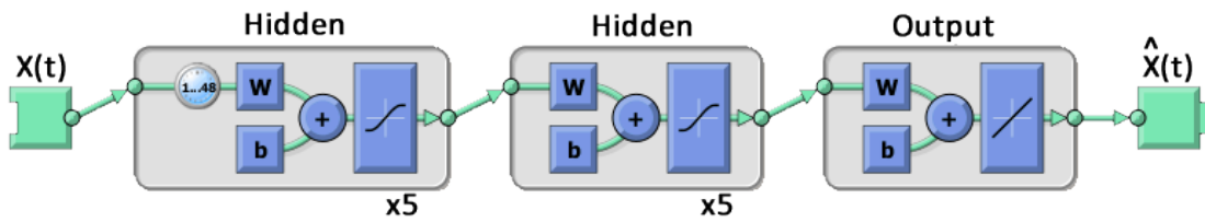
Figure 9- ANN for weather forecast
