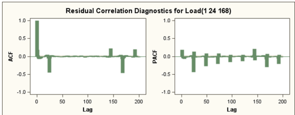
Figure 6- Residual analysis after the estimation of the transfer function model without any ARMA component
