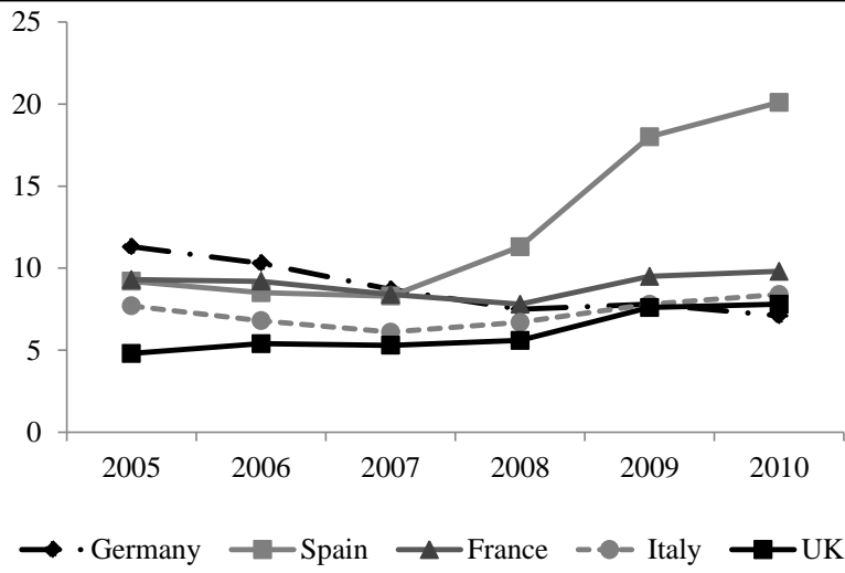
Figure 3 Unemployment rates, 2000-2010
