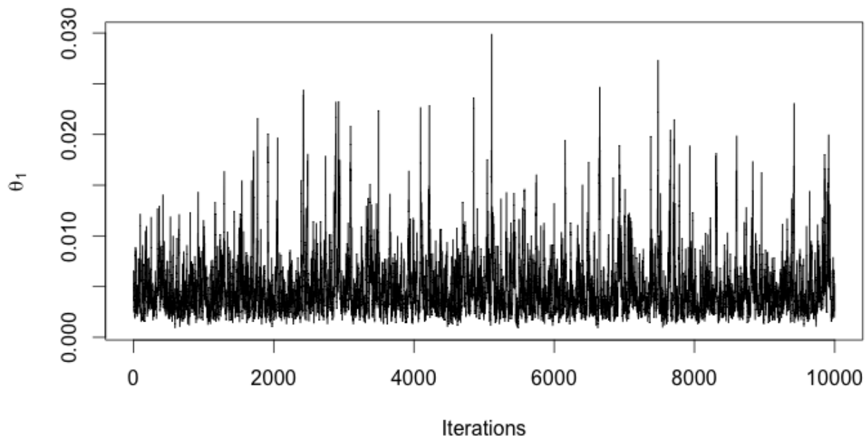
Figure 7: Trace Plot.
