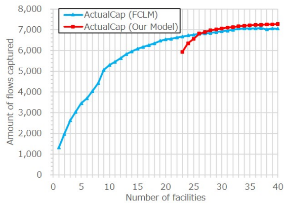
Figure 11: Transition of the values of ActualCap in N2
