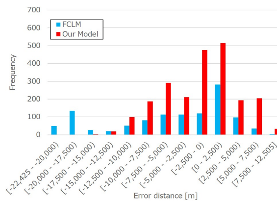
Figure 13: Distribution of the error distance by each model in N1
