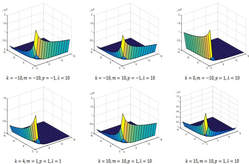
Fig. 1: 3D Plots of gamma function with six parameters k, n, r, m, p and \lambda
