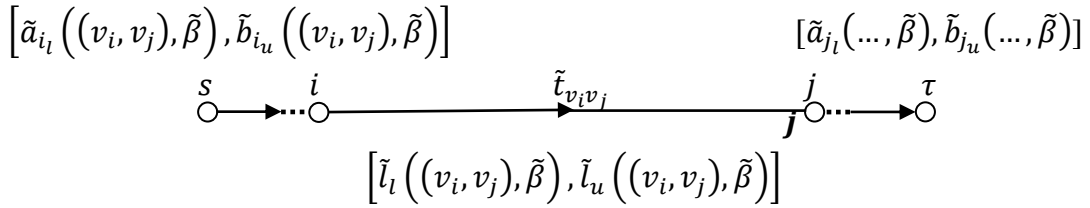
Figure 7: A network of \tilde{l} - \tilde{\beta} fuzzy interval minimum fuzzy cost fuzzy flow of the fuzzy time-widows problem
