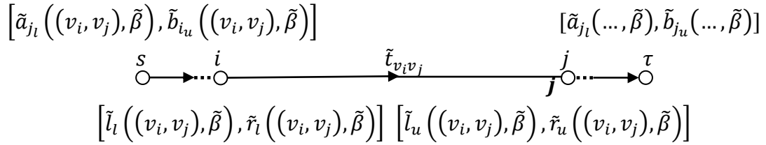
Figure 6: A network with fuzzy time-widows, fuzzy bounds and fuzzy flows
