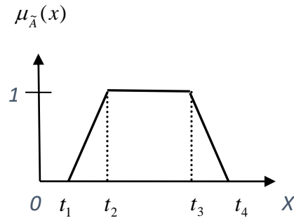
Figure 2: 4-Points representation of fuzzy interval
