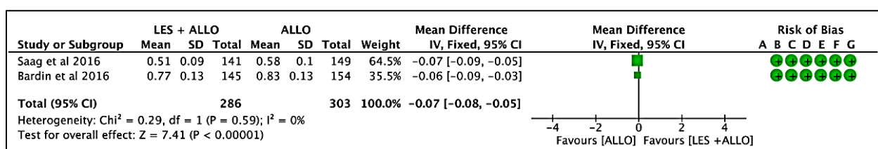
Fig. 1. Reduction in serum uric acid less than 6 mg/dL in lesinurad group versus allopurinol group during the follow-up
