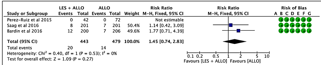
Fig. 4. Any serious Treatment Emergent Adverse Events (TEAEs) occur in lesinurad group versus allopurinol group during follow-up period
