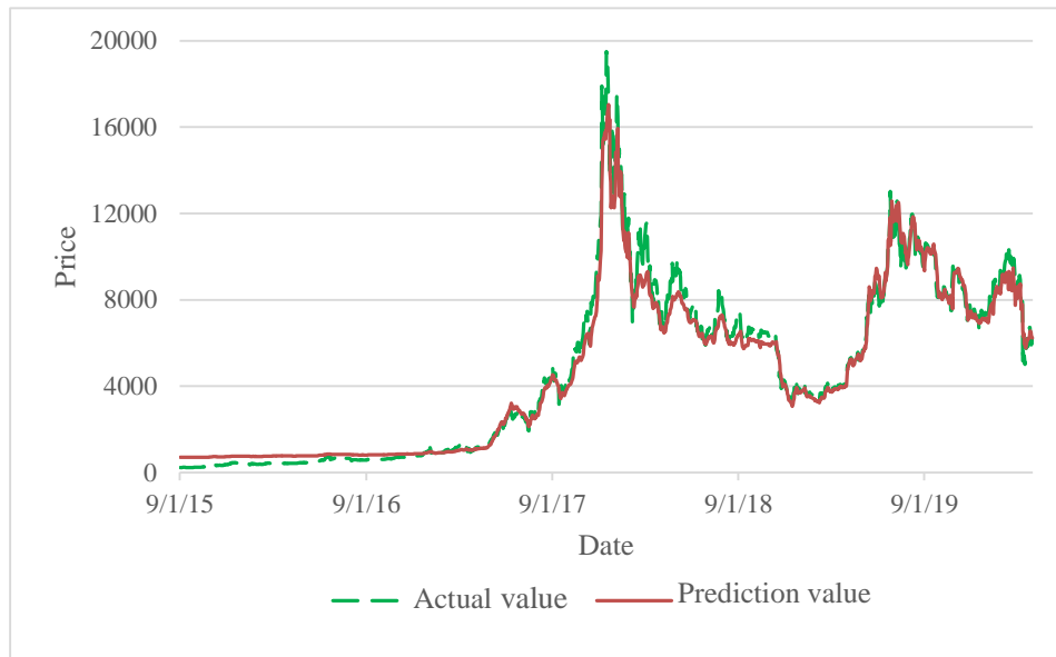
Figure 1. Prediction trend of the best BPNN with one hidden layer (2-4-1) under training.
