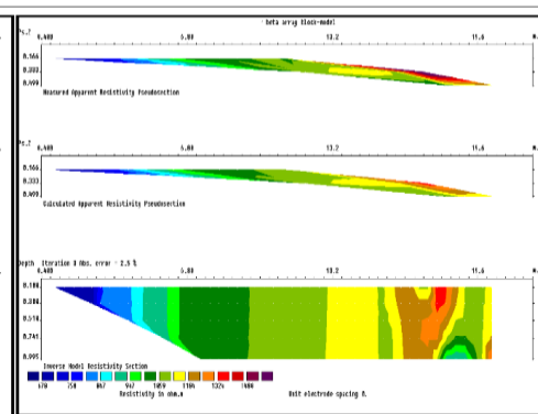
Fig. 15: 2D Resistivity Tomogram for Profile COT2
