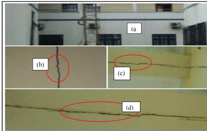
Plate 4: COLLEGE OF SCIENCE BUILDING showing the dangers of vertical and horizontal cracks on some parts of the building (a) shows part of the building under study (b) shows some vertical cracks (c) and (d) show some horizontal cracks.
