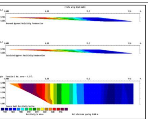
Fig.7: 2D Resistivity Tomogram for Profile ADM2
