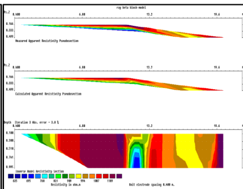
Fig. 17: 2D Resistivity Tomogram for Profile COT4
