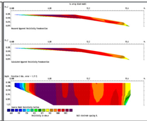
Fig. 5: 2D Resistivity Tomogram for Profile LIB4
