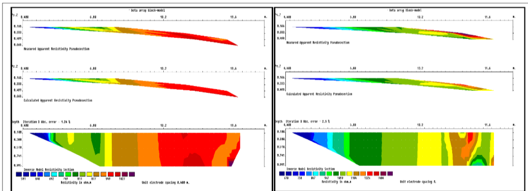
Fig. 14: 2D Resistivity Tomogram for Profile COT1
