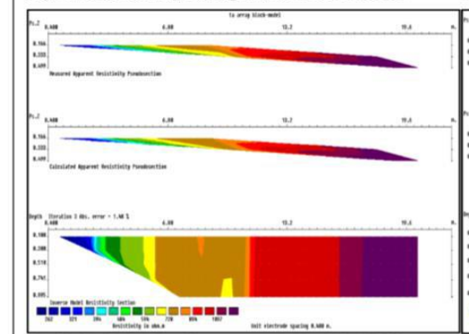
Fig. 8: 2D Resistivity Tomogram for Profile ADM3
