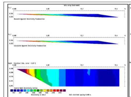
Fig. 6: 2D Resistivity Tomogram for Profile ADM1
