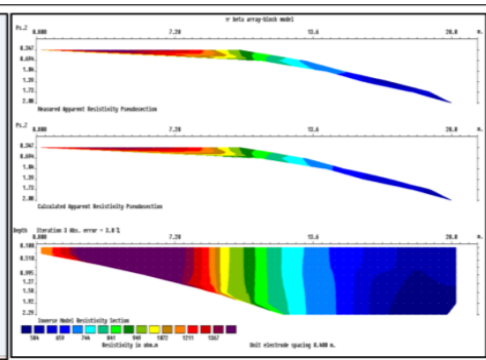
Fig.3: 2D Resistivity Tomogram for Profile LIB2
