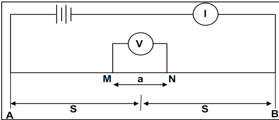
Figure 2: Schematic of Schlumberger array for data acquisition
