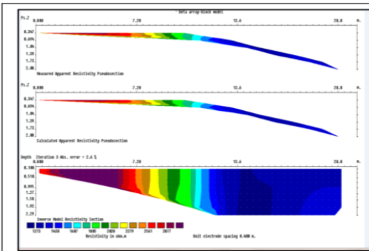
Fig. 2: 2D Resistivity Tomogram for Profile LIB1
