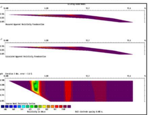
Fig. 9: 2D Resistivity Tomogram for Profile ADM4
