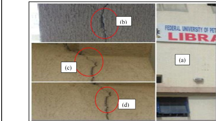
Plate 2: LIBRARY BUILDING showing the dangers of some severe vertical cracks at some parts of the building (a) shows part of the building under study (b) shows some vertical cracks at the upstairs (c) and (d) show some vertical cracks at the downstairs.
