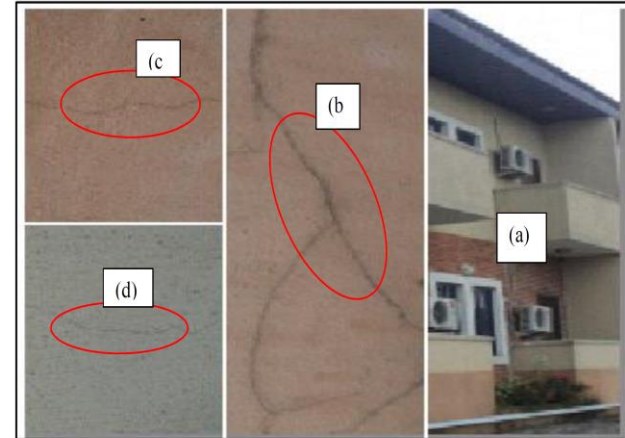
Plate 5: COLLEGE OF TECHNOLOGY BUILDING showing danger of some diagonal and horizontal cracks on some parts of the building; (a) shows parts of the building under study (b) shows some diagonal cracks (c) and (d) show some horizontal cracks.
