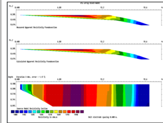
Fig. 4: 2D Resistivity Tomogram for Profile LIB3
