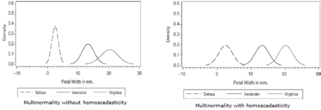
Figure 2: Discriminant Analysis of Fisher (1936) Iris data
