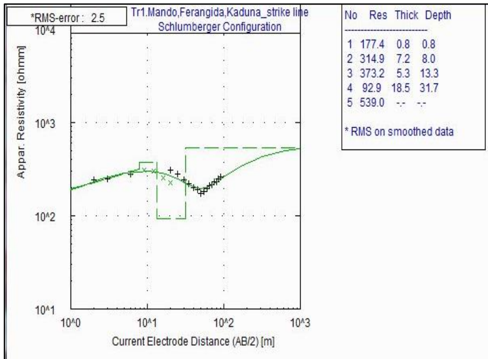
Figure 3: Geoelectric Section for Traverse 1
