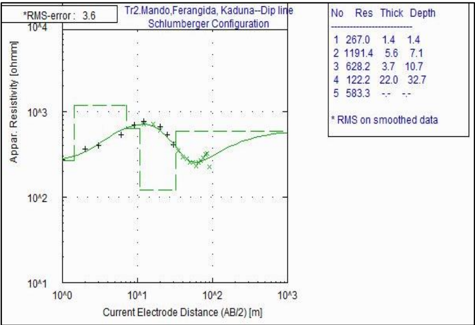
Figure 4: Geoelectric Section for Traverse 2
