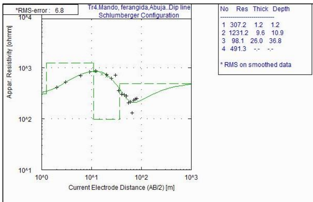
Figure 6: Goelectric Section for Traverse 4
