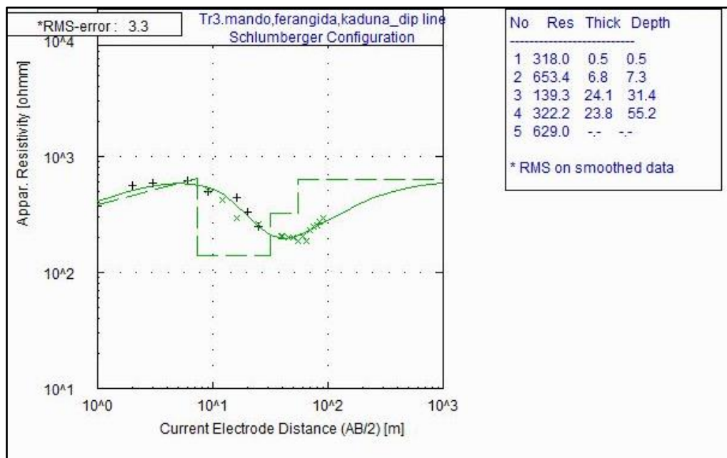
Figure 5: Goelectric Section for Traverse 3
