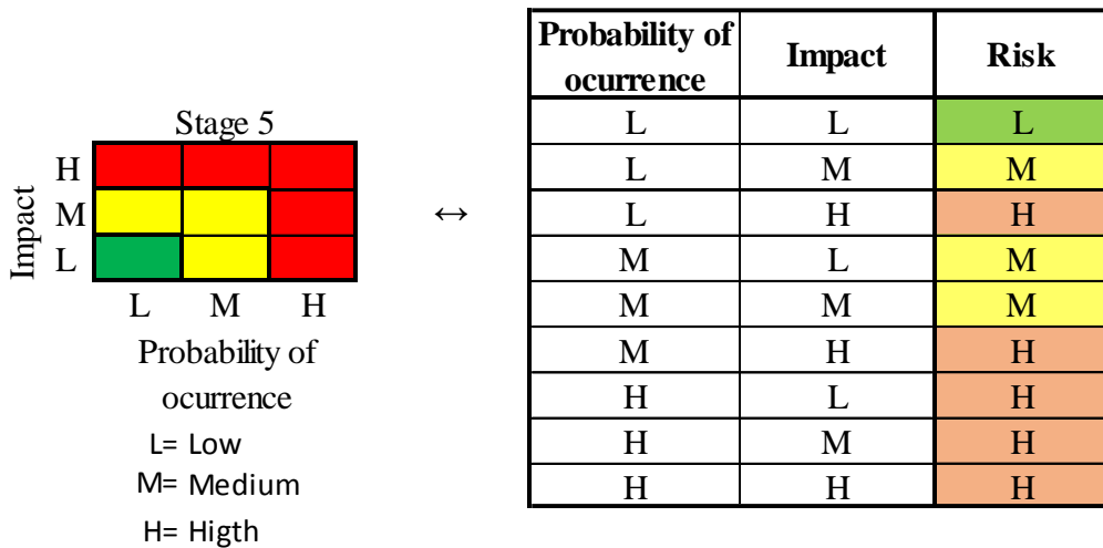
Figure 5: Risk Matrix
