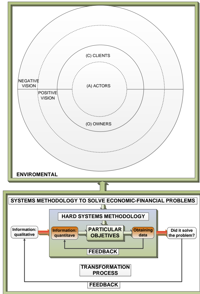
Figure 4: CATWOE Schematize
